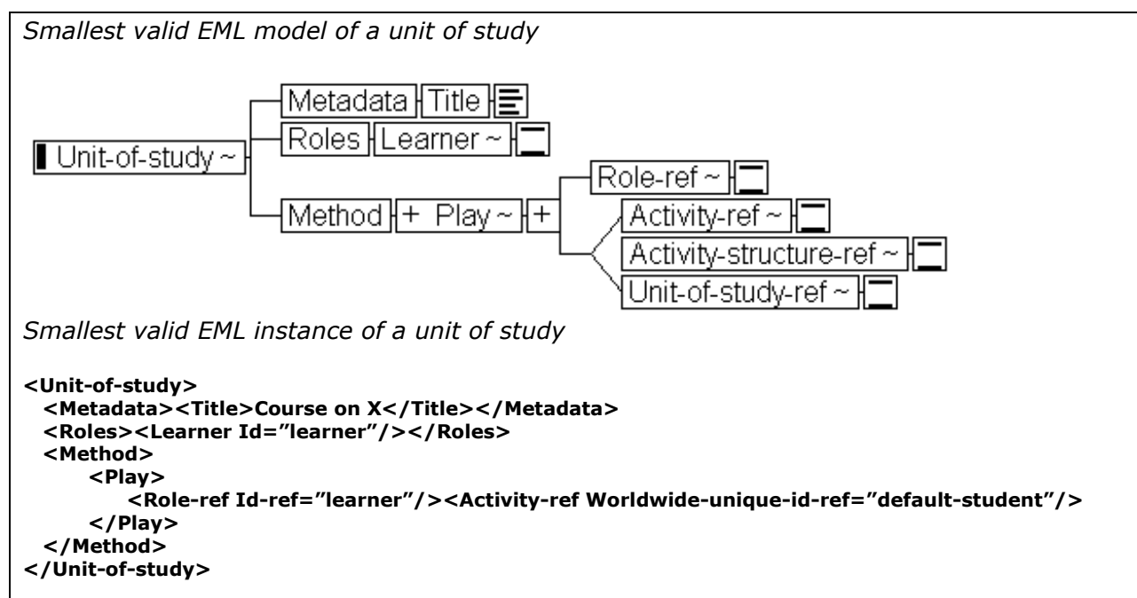
Figure 10. Smallest EML model of a unit of study and an example of a document instance.
